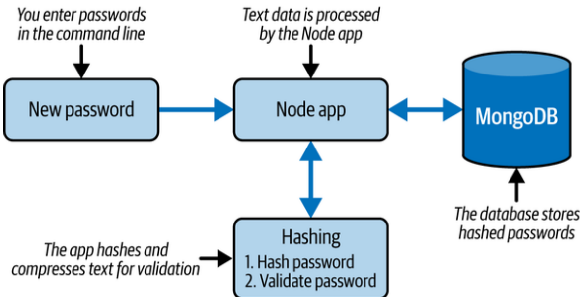
Figure 4-1. Project blueprint for flow of data in password manager app
