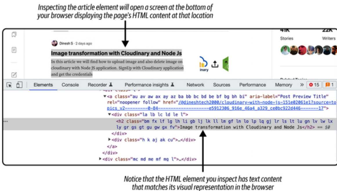
Figure 9-5. Example HTML page breakdown
