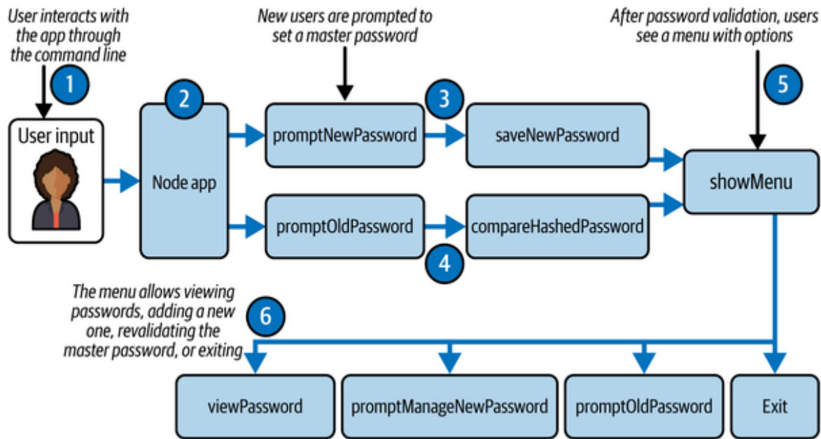
Figure 4-3. Code logic-flow diagram
